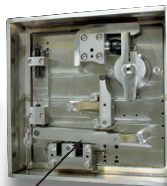
Open Valve
